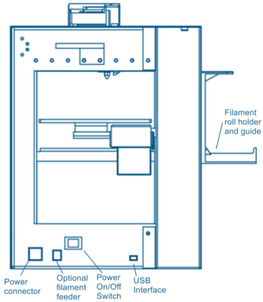
Figure 2. Back view of printer
